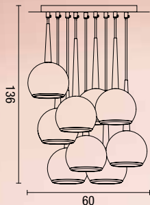
sospensione Bol 9 luci Bol pendant lamp 9 lights 2316 lampadine lighting 9 x E27 57W lampadine non incluse bulbs not included
