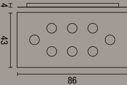
plafoniera Flet rettangolare 8 luci Flet rectangular ceiling lamp with 8 lights
