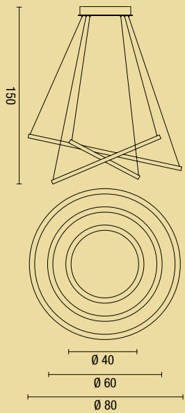
sospensione Aluring triplo anello Aluring triple rings pendant lamp
