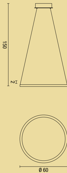
sospensione rotonda Aluring piccola Aluring round pendant lamp small
