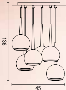
sospensione Bol 6 luci Bol pendant lamp 6 lights 2314 lampadine lighting 6 x E27 57W lampadine non incluse bulbs not included
