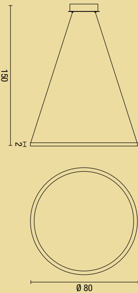
sospensione rotonda Aluring grande Aluring round pendant lamp large
