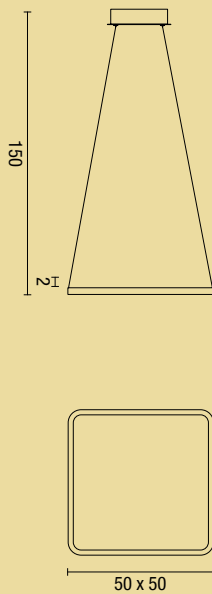
sospensione quadrata Aluring piccola Aluring square pendant lamp small
