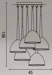
sospensione Bell 6 luci Bell pendant lamp 6 lights 2322 lampadine lighting 6 x E27 57W lampadine non incluse bulbs not included
