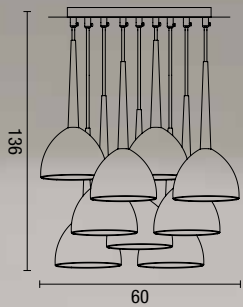
sospensione Bell 9 luci Bell pendant lamp 9 lights 2324 lampadine lighting 9 x E27 57W lampadine non incluse bulbs not included
