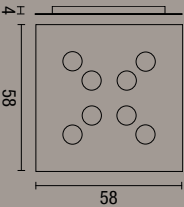
plafoniera Flet 8 luci Flet ceiling lamp with 8 lights
