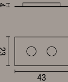
plafoniera Flet rettangolare 2 luci Flet rectangular ceiling lamp with 2 lights
